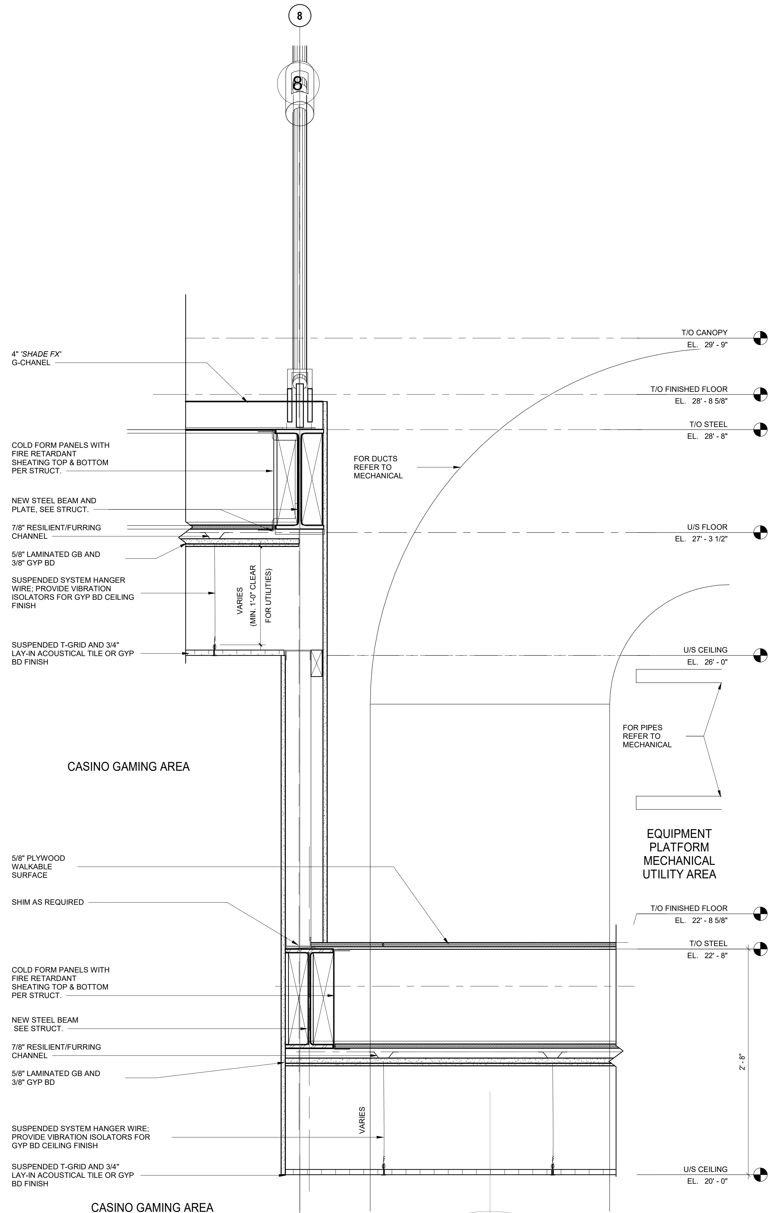
6 CEILING DETAIL AT PLATFORM TRANSITION SCALE: 1 1/2" = 1'-0"
