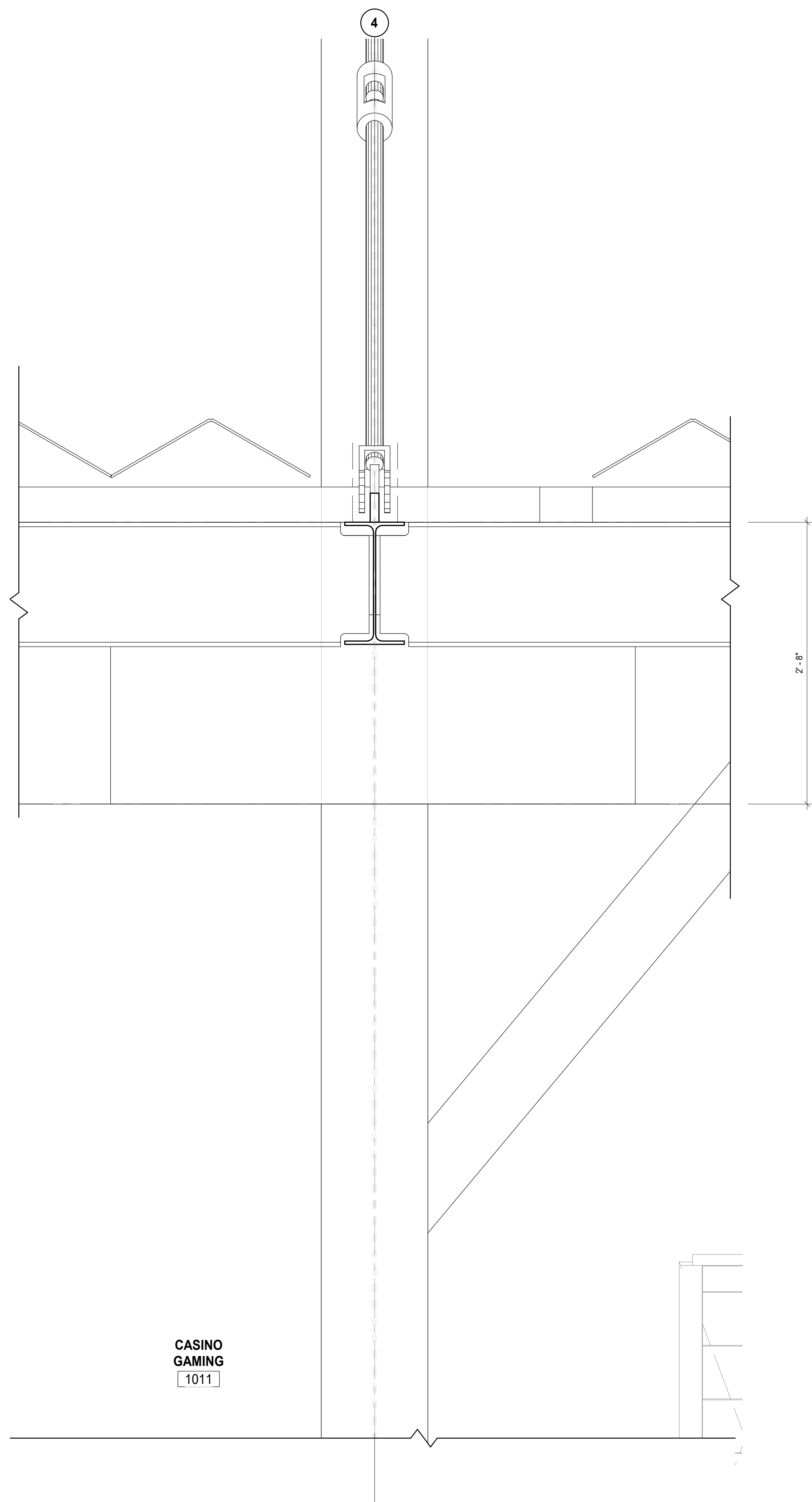
7 SECTION DETAIL AT EQUIPMENT PLATFORM SCALE: 1 1/2" = 1'-0"
