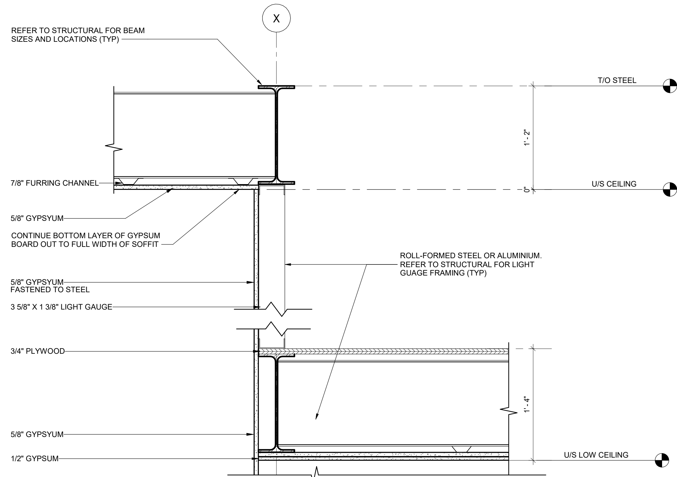
4 CEILING DETAIL - METAL LINEAR CEILING SYSTEM CARRIER AT RECEPTION - 'KNEE-WALL' (TYPICAL) SCALE: 1 1/2" = 1'-0"
