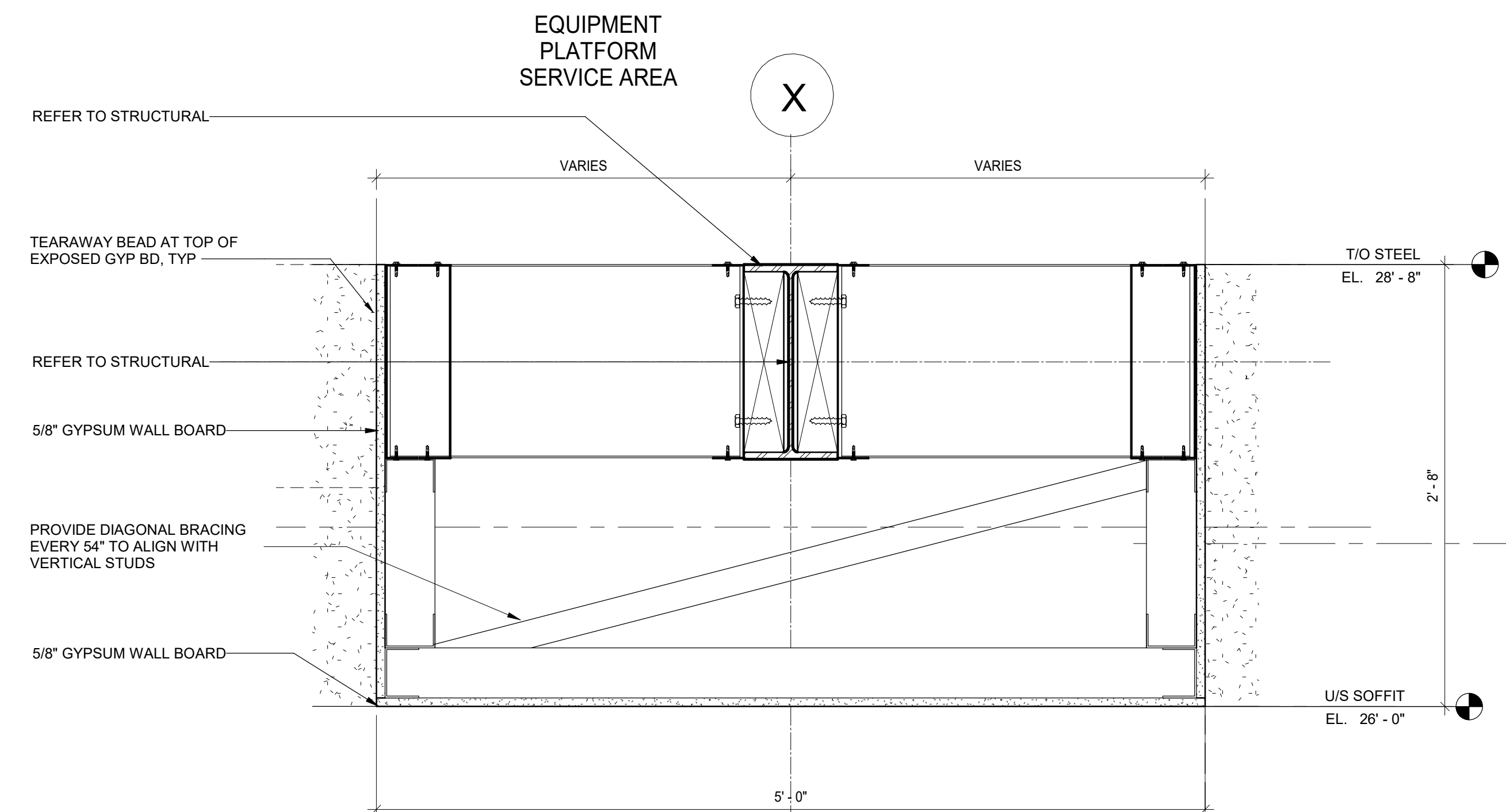
5 CEILING DETAIL AT SOFFIT (TYPICAL) SCALE: 1 1/2" = 1'-0"
